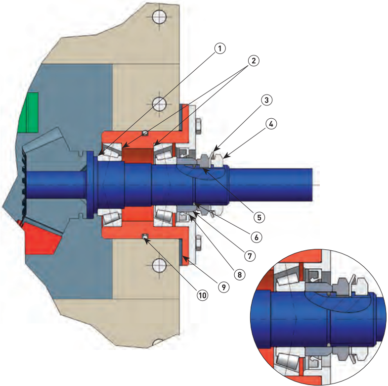
figure 6 O-application of bearing, free of clearance or prestressed (supporting effect outside of the bearing)
